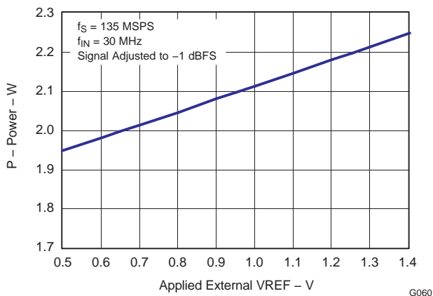
Figure 65. Total Power Consumption versus External VREF
